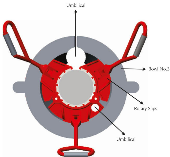
Umbilical Bowl & Rotary Slips Figure No. 39
