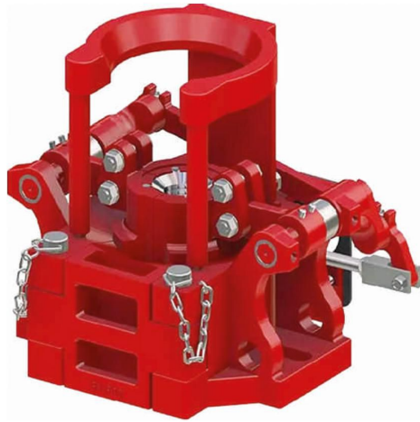
Pneumatic Tubing Spiders Figure No. 25
