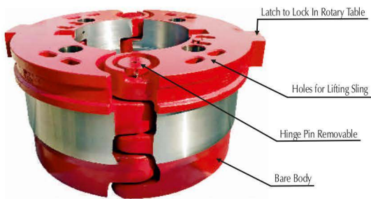
Master Bushing for National RT Model : ABMB 3750 Figure No. 1
