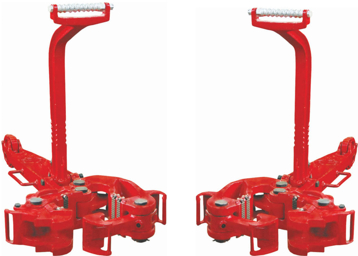
Manual Tongs Figure No. 24
