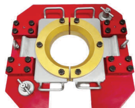
Wear Guide Assembly Figure No. 17
