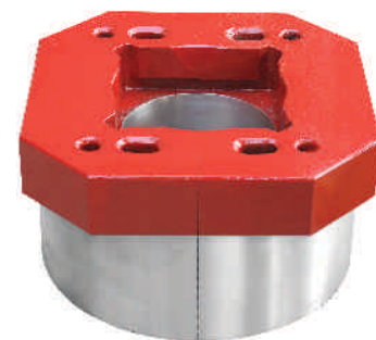
27.1/2" Split & Inbuilt Taper Master Bushing Figure No. 11
