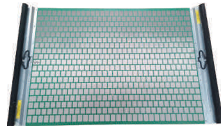
Screen for SuperFlow Shale Shakers Model : SCREEN SF-A Figure No. 48
