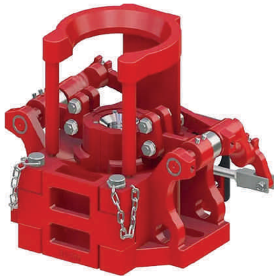
Pneumatic Tubing Spiders Figure No. 25
